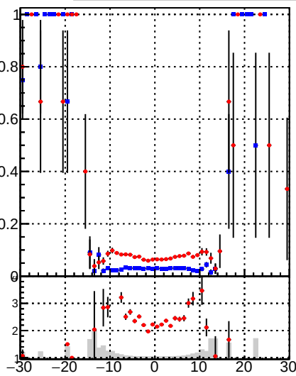
—•— DQM_mkFit —•— DQM_BDT_mkFit
