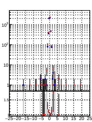
N of associated (recoToSim) loop tracks vs dxy(PV)
