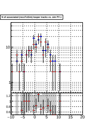
N of reco track vs. sim PV z
