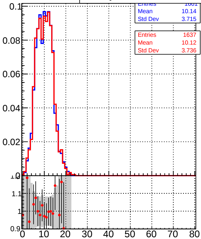
Legend: DQM_mkFit (blue line with squares), DQM_BDT_mkFit (red line with circles)
