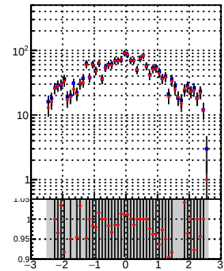
N of reco track vs \eta Legend: DQM_mkFit (blue stars) DQM_BDT_mkFit (red stars)
