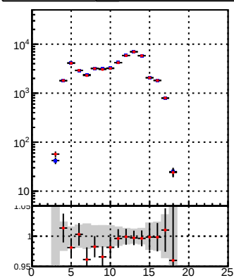
N of reco track vs hit DQM_mkFit DQM_BDT_mkFit
