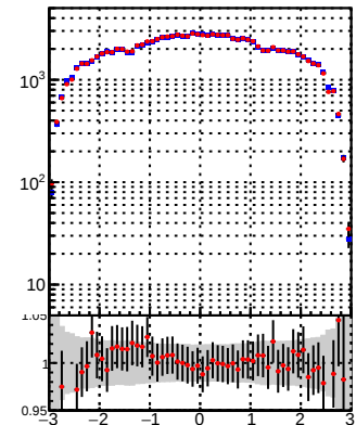
N of reco track vs \eta DQM_mckFit DQM_BDT_mckFit
