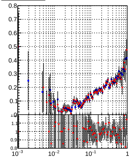
Fake rate vs \epsilon Legend: DQM_mkFit (blue line with markers) DQM_BDT_mkFit (red line with markers)
