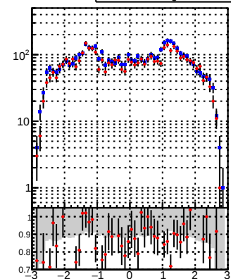
N of reco track vs \eta —•— DQM_mkFit —•— DQM_BDT_mkFit
