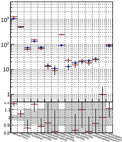
Number —●— DQM_BDT_mkFit
