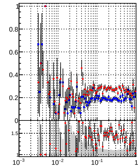
—•— DQM_mkFit —•— DQM_BDT_mkFit
