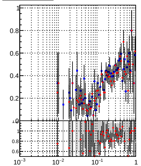
Legend: DQM_mkFit (blue line with markers), DQM_BDT_mkFit (red line with markers)
