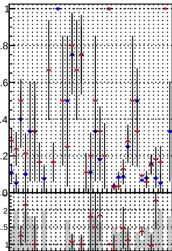
Fake rate vs. —●— DQM_mkFit —●— DQM_BDT_mkFit
