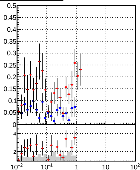
—•— DQM_mkFit —•— DQM_BDT_mkFit
