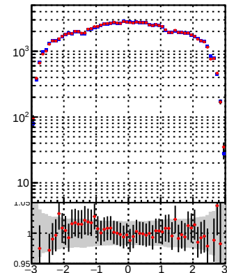
—•— DQM_mkFit —•— DQM_BDT_mkFit
