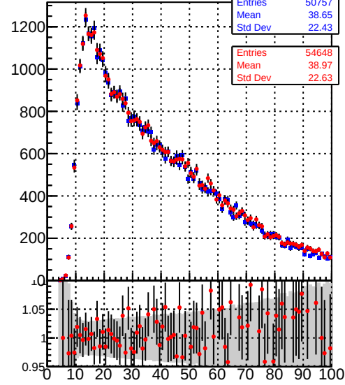
Uncertainty x Coordinate (other Vtx) Legend: DQM_mkFit (blue line), DQM_BDT_mkFit (red line)
