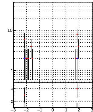
N of associated (recoToSim) duplicate tracks vs \eta —•— DQM_mkFit —x— DQM_BDT_mkFit
