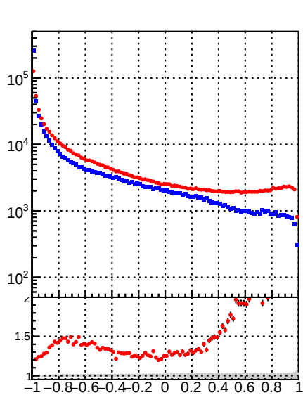
Efficiency (tracking eff factorized out) vs. MVA1
