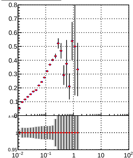
—•— DQM_mkFit —•— DQM_BDT_mkFit
