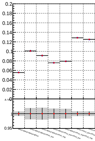
Fake rate vs. Legend for the bottom row plots: —•— DQM_mkFit —•— DQM_BDT_mkFit
