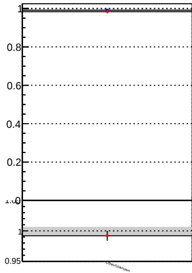
Fake rate vs. DQM_mkFit DQM_BDT_mkFit
