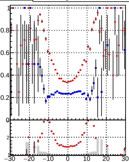
—•— DQM_mkFit —•— DQM_BDT_mkFit
