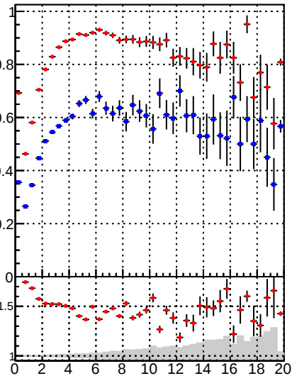
Fake rate vs. —●— DQM_mkFit —●— DQM_BDT_mkFit
