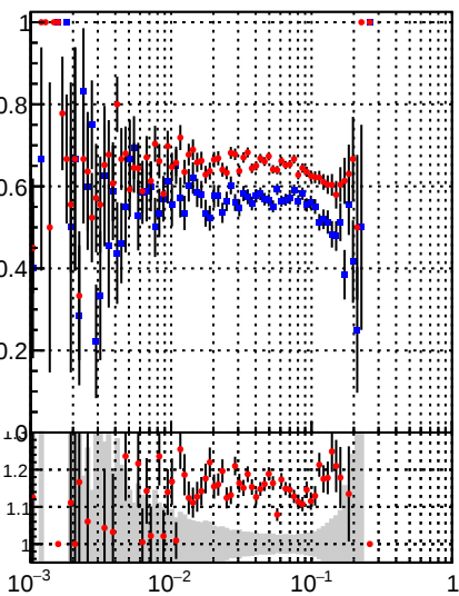
—•— DQM_mkFit —•— DQM_BDT_mkFit
