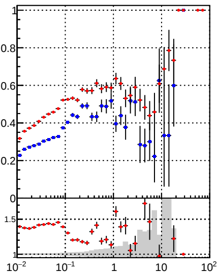
—•— DQM_mkFit —•— DQM_BDT_mkFit
