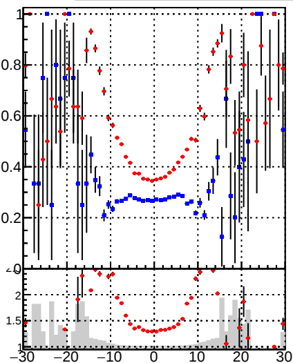
—•— DQM_mkFit —•— DQM_BDT_mkFit
