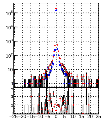
—•— DQM_mkFit —•— DQM_BDT_mkFit
