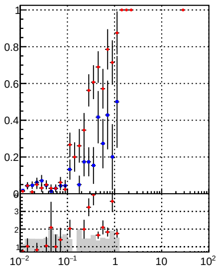
—•— DQM_mkFit —•— DQM_BDT_mkFit
