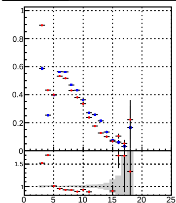
Fake rate vs hit Legend: DQM_mkFit (blue circles), DQM_BDT_mkFit (red circles)
