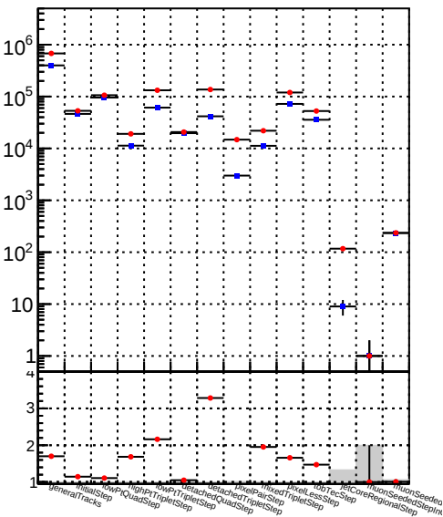
Number of tracks vs collection Legend: DQM_CKF (blue), DQM_BDT_CKF (red)
