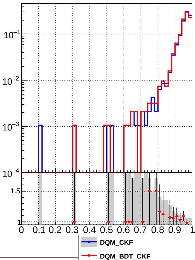
RecoPVAssoc2GenPVMatched_Missing
