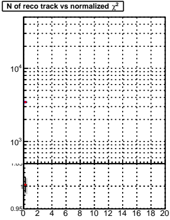
N of reco track vs. \chi^2 Legend: DQM_CKF (Blue line) DQM_BDT_CKF (Red line)
