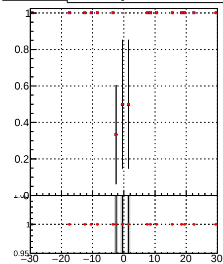
Fake rate vs \eta
