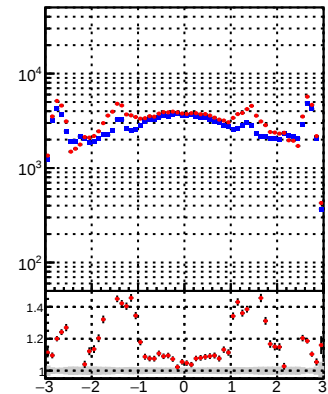
N of reco track vs \eta pT eta Legend: —•— DQM_CKF —•— DQM_BDT_CKF
