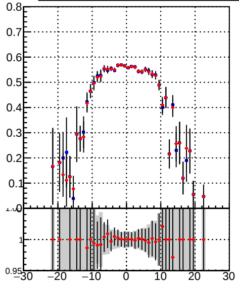
Efficiency vs. sim PV z Legend: — DQM_CKF (blue line with dots) — DQM_BDT_CKF (red line with dots)
