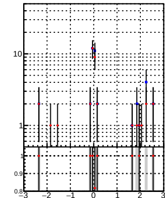
N of associated (recoToSim) duplicate tracks vs \eta —•— DQM_CKF —•— DQM_BDT_CKF
