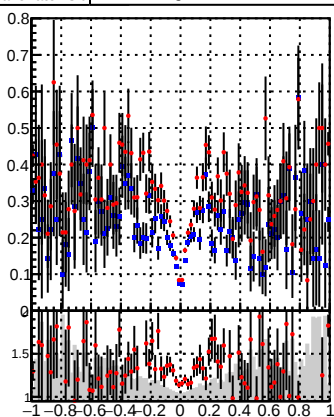
Fake rate vs d
