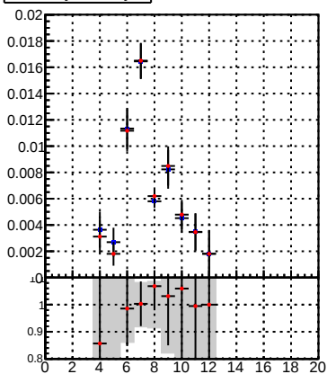
Efficiency vs 3D layer (continued)
