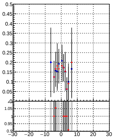
Fake rate vs d Legend: DQM_CKF (blue dots) DQM_BDT_CKF (red dots)
