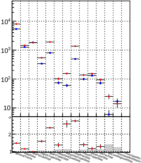
Number —●— DQM_BDT_CKF
