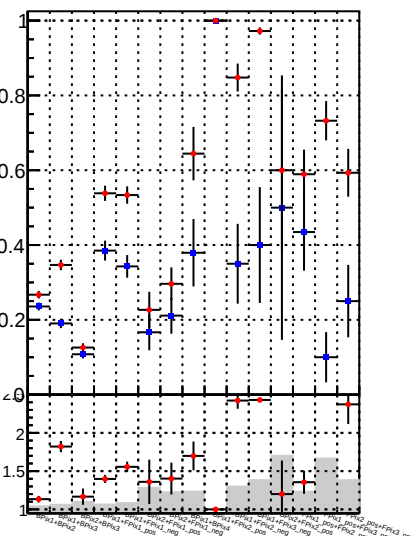
Fake rate vs. —●— DQM_CKF —●— DQM_BDT_CKF
