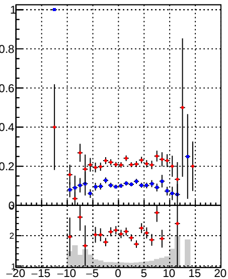
fake+duplicates vs Sim. PV z
