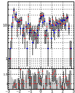
N of reco track vs \eta Legend: DQM_CKF (blue diamonds) DQM_BDT_CKF (red crosses)
