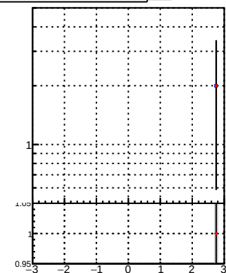
N of associated (recoToSim) duplicate tracks vs \eta Legend: DQM_CKF (blue diamonds) DQM_BDT_CKF (red circles)
