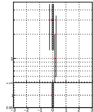
N of associated (recoToSim) duplicate tracks vs \eta DQM_BDT_CKF
