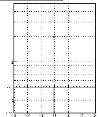
N of associated (recoToSim) duplicate tracks vs \eta DQM_CKF
