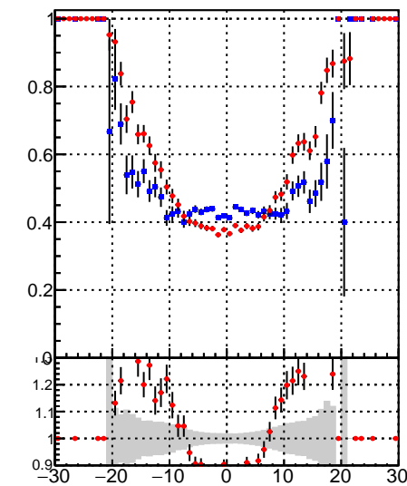
Fake rate vs d —●— DQM_CKF —●— DQM_BDT_CKF
