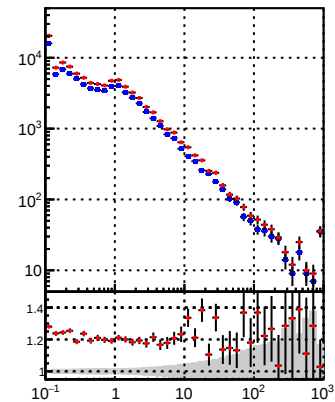
N of reco track vs e
