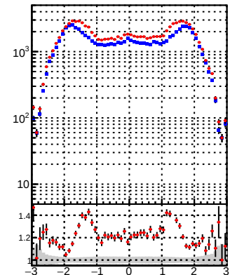
N of reco track vs e
