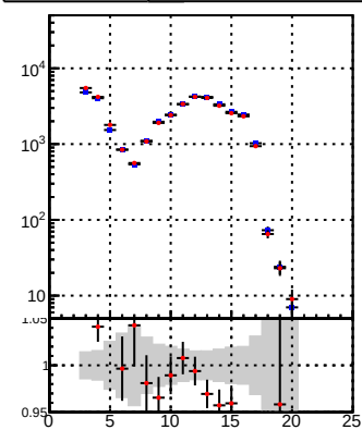
N of reco track vs hit DQM_CKF DQM_BDT_CKF
