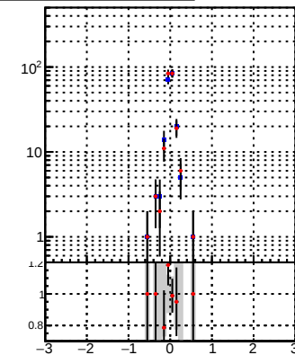
N of associated (recoToSim) tracks vs \eta Legend: DQM_CKF (blue diamonds) DQM_BDT_CKF (red crosses)
