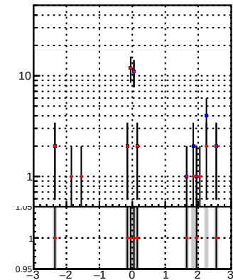
N of associated (recoToSim) tracks vs \eta —•— DQM_CKF —•— DQM_BDT_CKF
